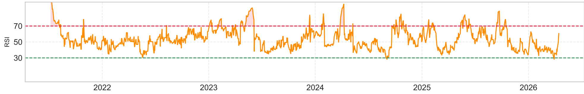
RSI (14-day) — Current: 60.8
