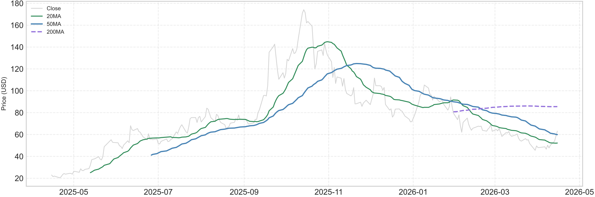
OKLO — Closing Price with Moving Averages (1 Year)
